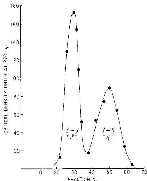
FIGURE 3: Ion-exchange chromatographic separation of tubercidinyl-(2'→5')-thymidine (TuP T) and tubercidinyl-(3'→5')-thymidine on a DEAE-cellulose carbonate column (18 × 21 cm). The gradient elution was 0.08–0.125 N (\text{C}_2\text{H}_5)_3\text{N}^+\text{H} \text{HCO}_3^- .
